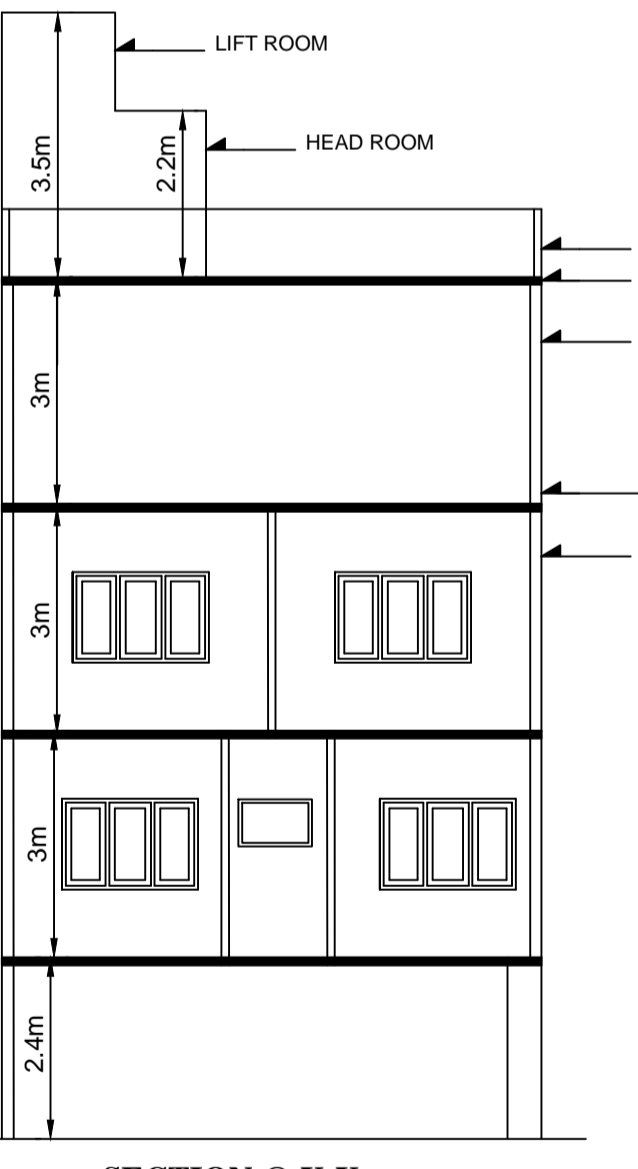
SECTION @ X-X
